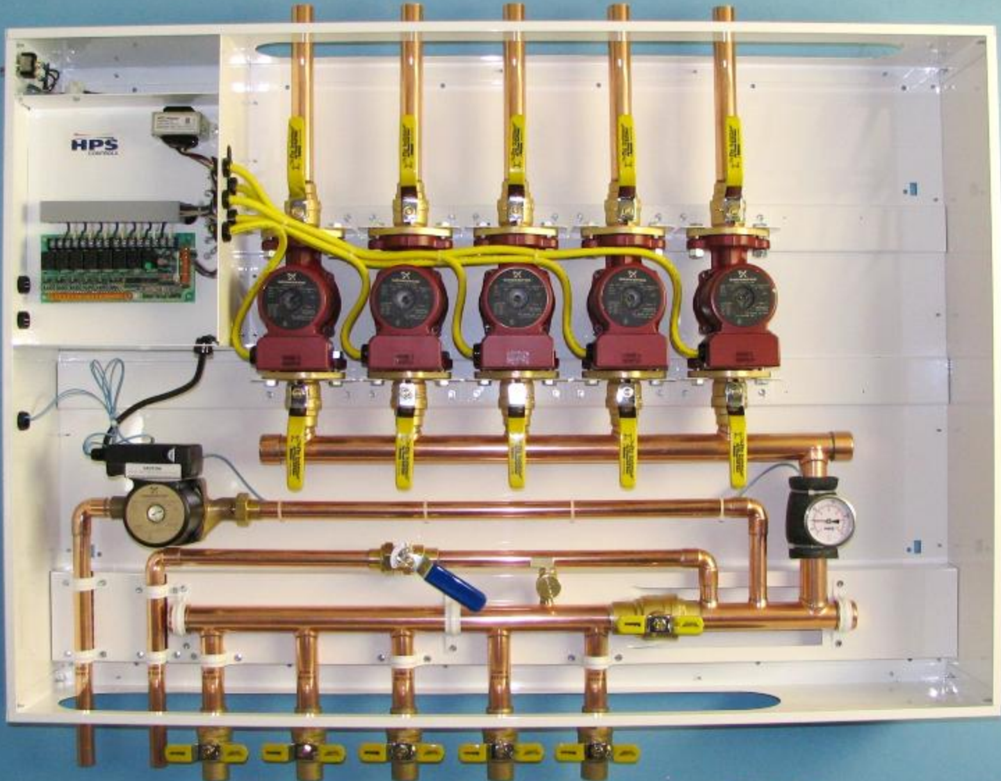
LFI-5 [Low Temp Injection 5 Zone Control Station]
